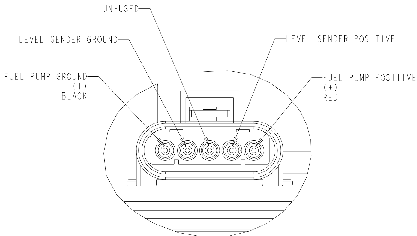
VIEW A E-CONN PIN OUT SCALE 2:1
